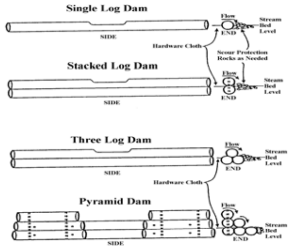
LOG DROP STRUCTURE DETAILS
